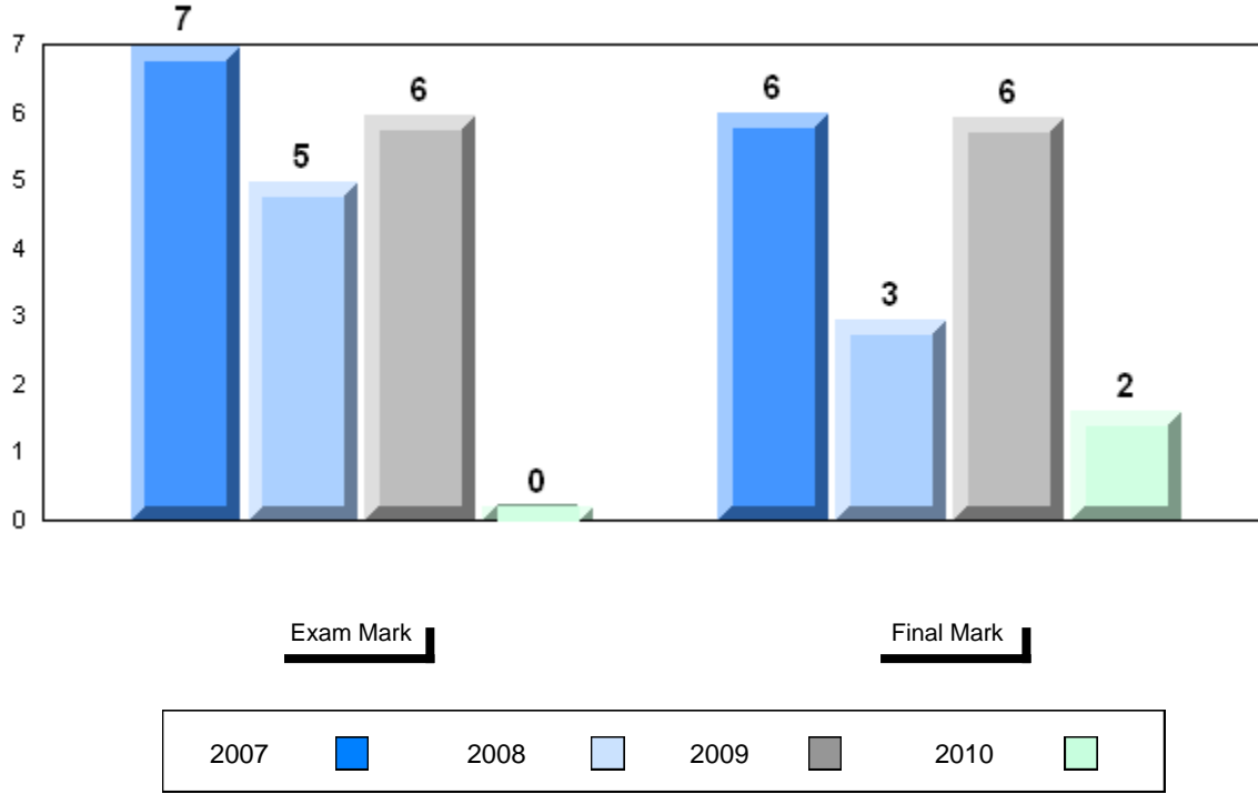
Difference from Provincial Mean, 2007-2010
