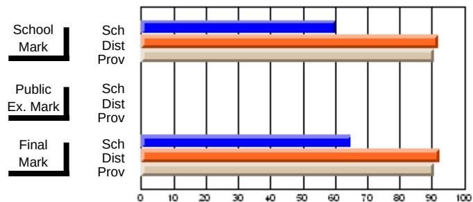
Percent Passes
