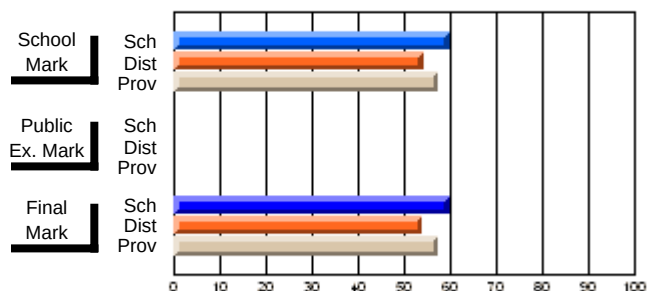
Average Scores
