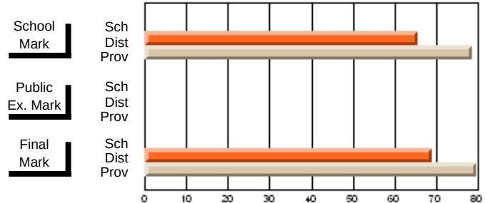
Percent Passes
