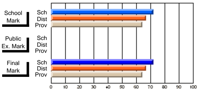
Average Scores
