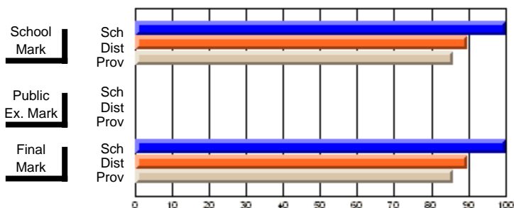
Percent Passes
